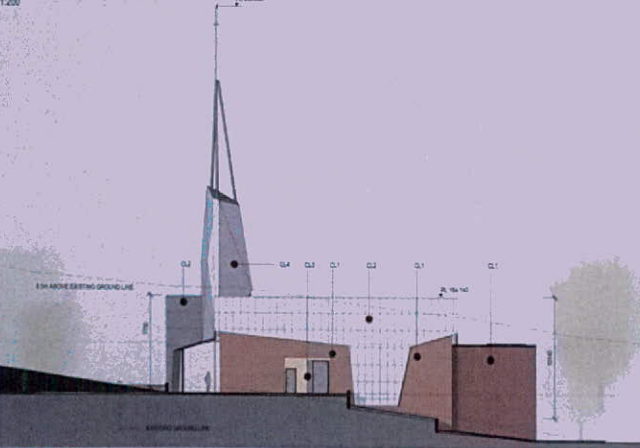
SOUTH WEST ELEVATION 1:200
