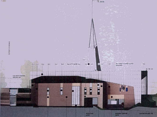
SOUTH EAST ELEVATION 1:200
